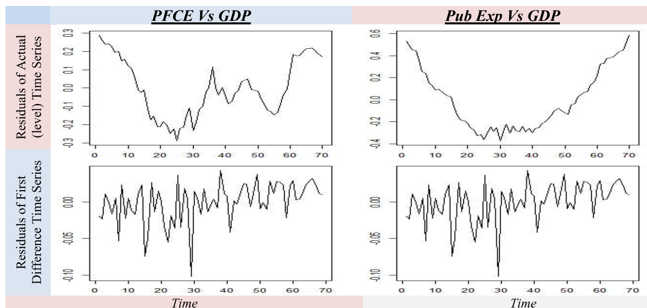
Figure 1: Signal-Spread of Residuals
